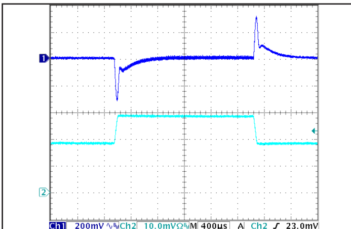
Figure 5: Output voltage response to step-change in load current (50% -75% -50% of Iout(max); dI/dt = 0.1 A/μs). Load cap: 1 μF ceramic and 15 μF tantalum capacitors. Ch 1: Vout (200 mV/div), Ch 2: Iout (5 A/div).
