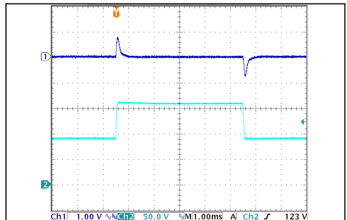
Figure 6: Output voltage response to step-change in input voltage (1000 V/ms). Load cap: 100 \mu F electrolytic output capacitance. Ch 1: V_{out} (1 V/div), Ch 2: V_{in} (50 V/div).
