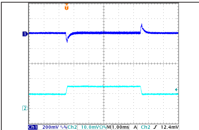
Figure 5: Output voltage response to step-change in load current (50% -75% -50% of Iout(max); di/dt = 0.1 \text{ A}/\mu\text{s} ). Load cap: 1 \mu\text{F} ceramic and 15 \mu\text{F} tantalum capacitors. Ch 1: Vout (200 mV/div), Ch 2: Iout (20 A/div).
