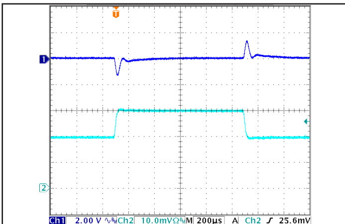
Figure 5: Output voltage response to step-change in load current (50% -75% -50% of I_{out(max)} ; dI/dt = 0.1 A/\mu s ). Load cap: 1 \mu F ceramic capacitor. Ch 1: V_{out} (2 V/div), Ch 2: I_{out} (2 A/div).
