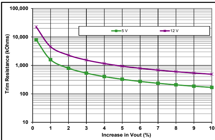
Common Figure 3: Trim graph for trim-up 5 to 12 V outputs.
