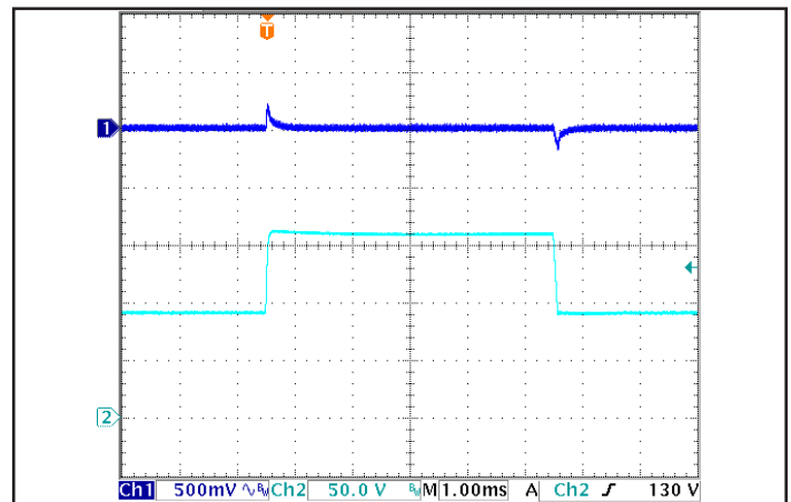
Figure 6: Output voltage response to step-change in input voltage (1000 V/ms). Load cap: 100 \mu\text{F} electrolytic output capacitance. Ch 1: Vout (500 mV/div), Ch 2: Vin (50 V/div).
