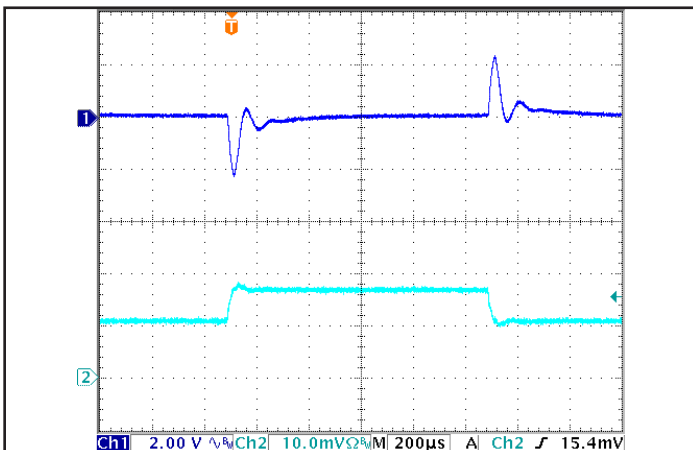
Figure 5: Output voltage response to step-change in load current (50% -75% -50% of I_{out(max)} ; dI/dt = 0.05 A/\mu s ). Load cap: 1 \mu F ceramic capacitor. Ch 1: V_{out} (2 V/div), Ch 2: I_{out} (2 A/div).
